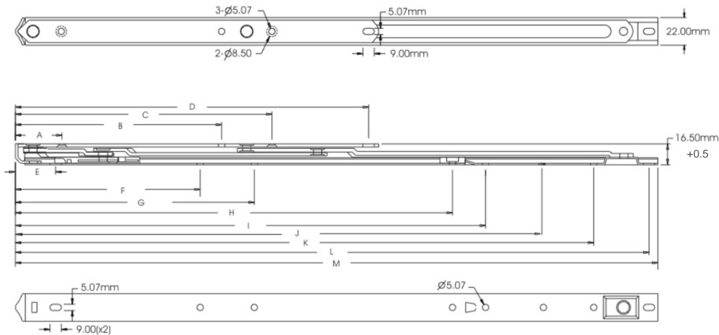
尺寸 MEASUREMENTS (mm)
