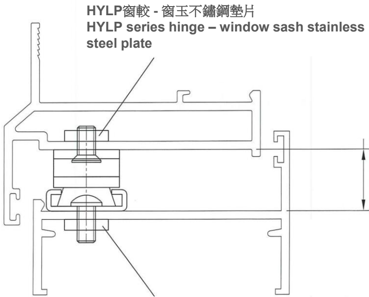
HYLP窗較 – 窗框不鏽鋼墊片 HYLP series hinge - window frame stainless steel plate
